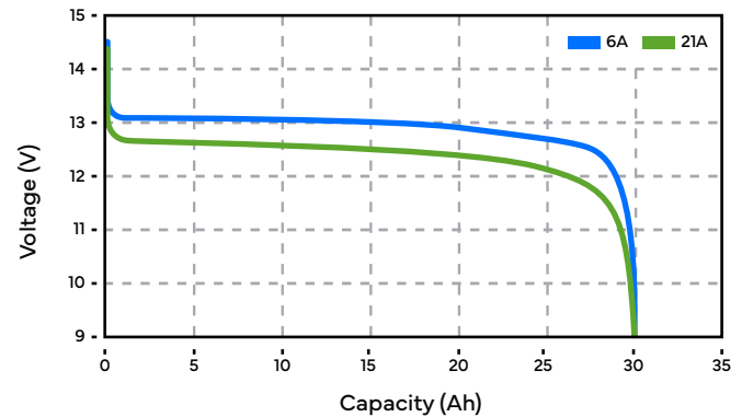
GTB24VU1-HC Discharge Rates at 25°C
