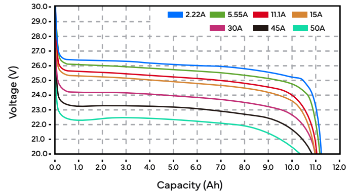
K2B12V22EB Discharge Rates at 23°C
